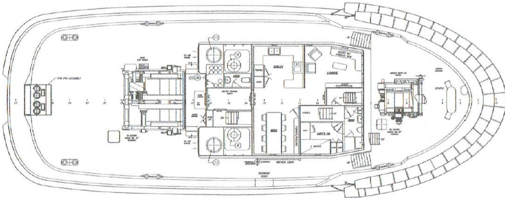
PLAN—MAIN DECK
